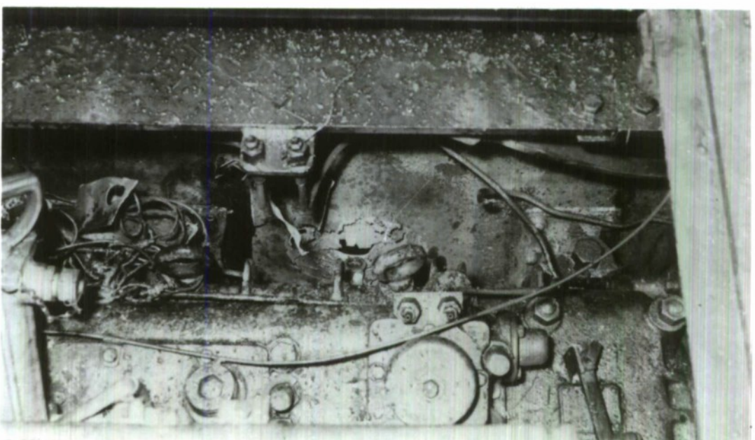
FIG. 14 DIRECT HIT ON REAR HULL PLATE
