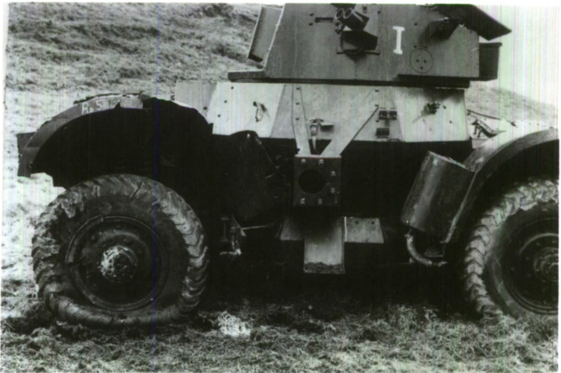
FIG. 5 DIRECT HIT ON WHEEL HUB
